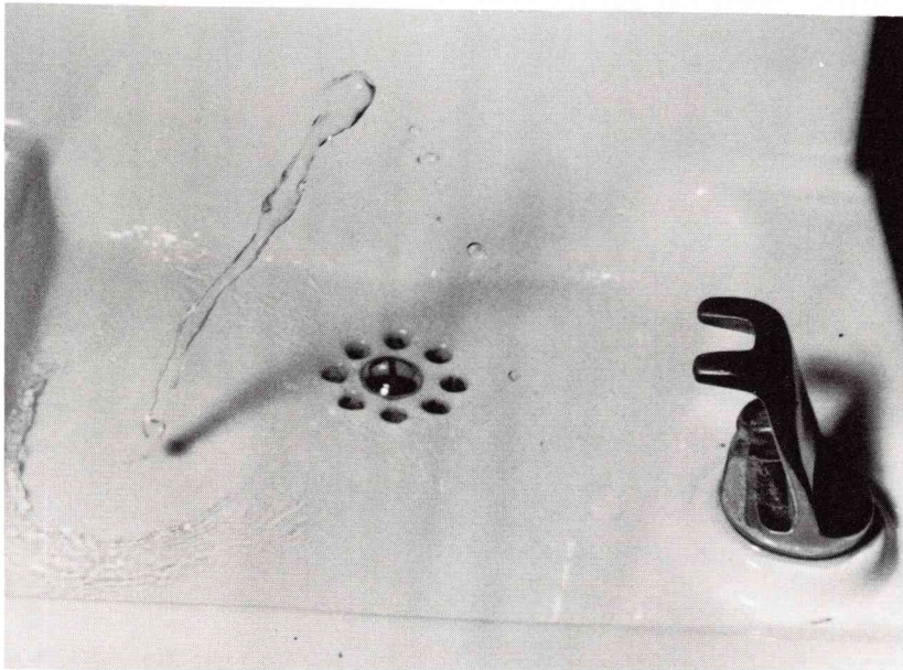
eruption
