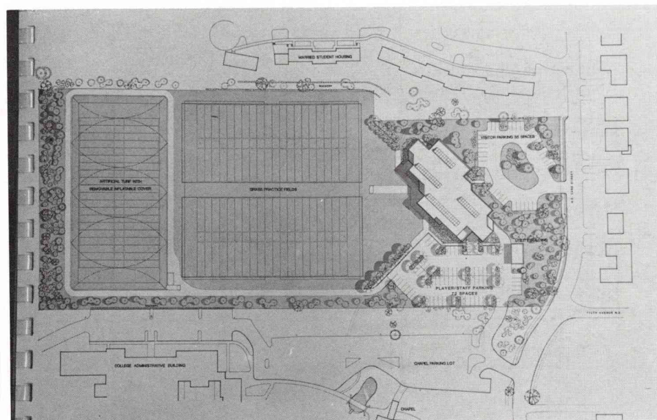
The Proposed Site Plan
